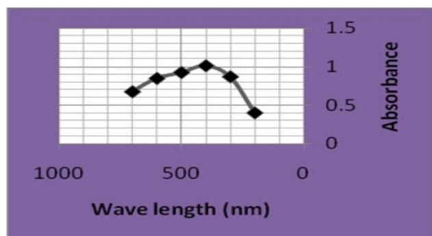
Figure 3: UV-Vis spectra of the ZnO NPs
