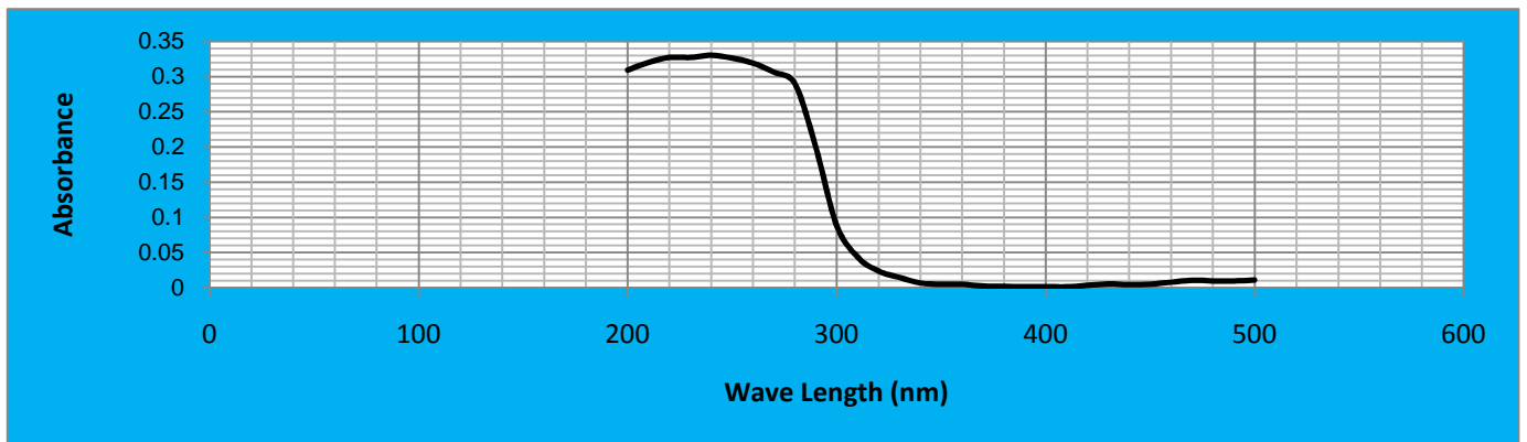
Figure 2: Absorbance spectra of the titanium dioxide nanoparticles
