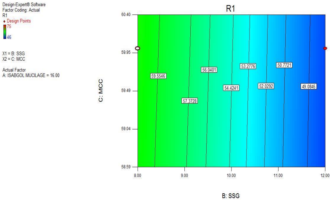
Figure No.15:- Contour plot showing Combined effect of MCC & SSG when Isabgol Mucilage kept at higher level i.e. 16mg.
