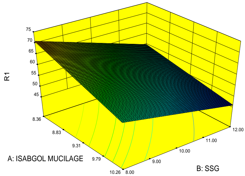
Figure No.06:- Response surface diagram showing combined effect of Isabgol mucilage & SSG when MCC kept at lower level i.e. 40 mg.
