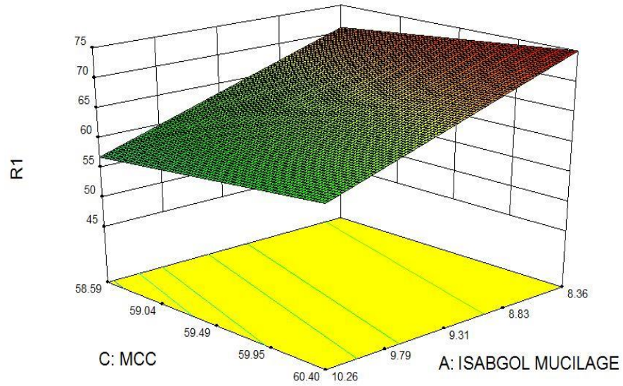
Figure No.10:- Response surface diagram showing Combined effect of MCC & Isabgol Mucilage when SSG kept at lower level i.e. 8 mg.
