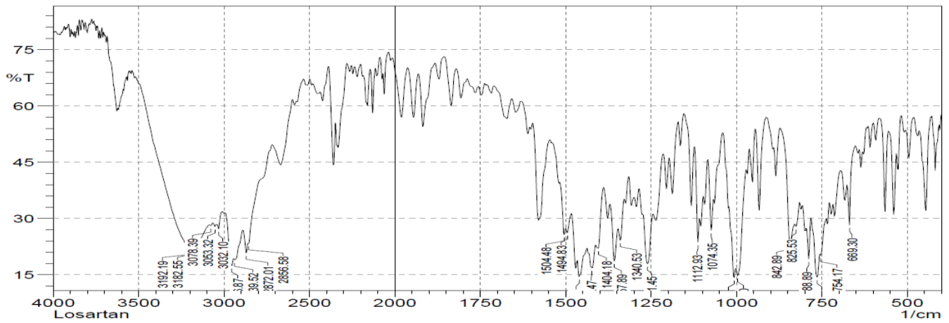
Figure No. 01:- FT-IR spectrum of Losartan potassium
