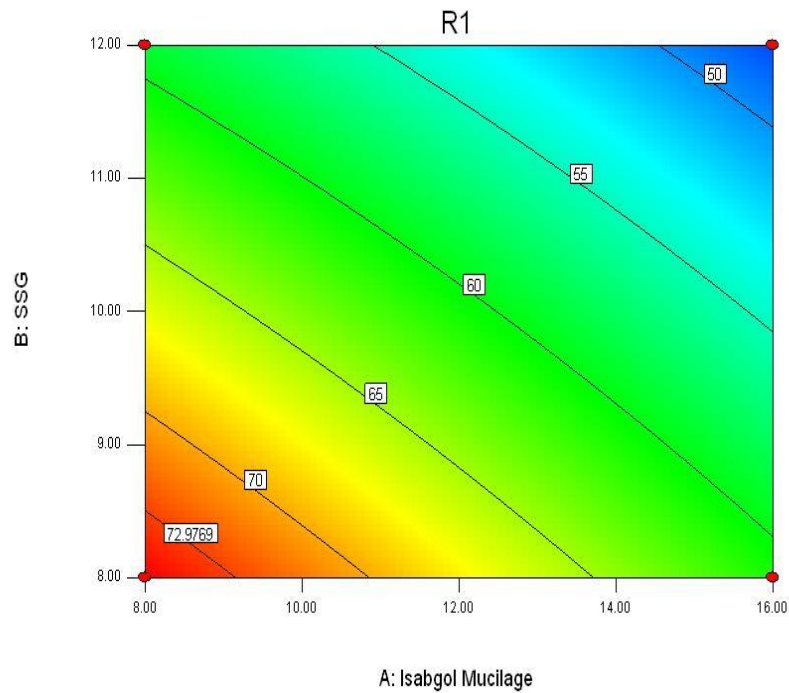
Figure No.13:- Contour plot showing combined effect of Isabgol mucilage & SSG when MCC kept at higher level i.e.60 mg.
