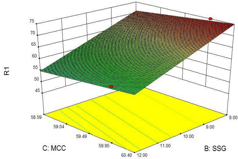
Figure No.08:- Response surface diagram showing Combined effect of MCC & SSG when Isabgol Mucilage kept at lower level i.e. 8 mg.
