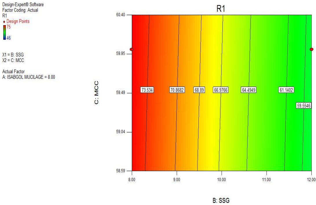
Figure No.14:- Contour plot showing Combined effect of MCC & SSG when Isabgol Mucilage kept at lower level i.e. 8 mg.
