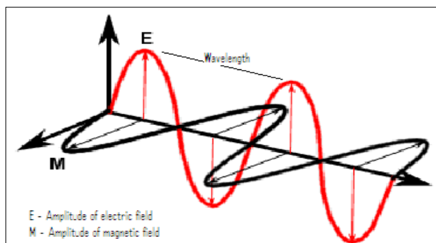
Fig.1. Electromagnetic wave in free space
