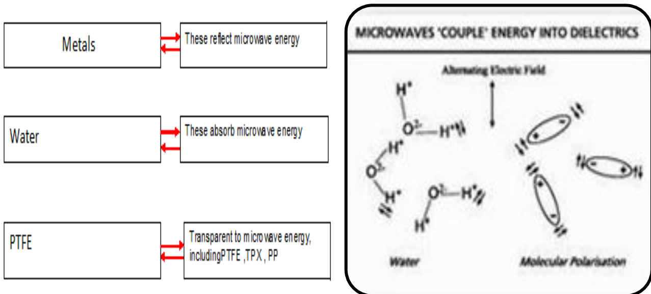
Fig.4. Di-pole rotation in a microwave field
